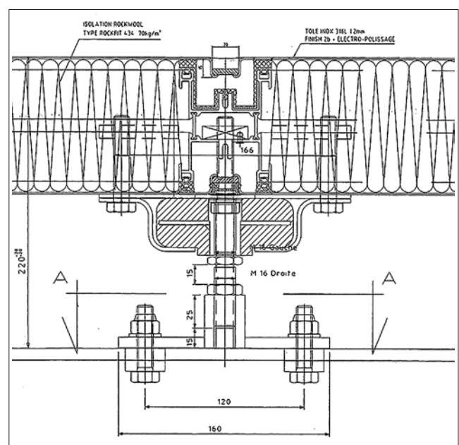
Fig. 4: Detail of the new skin, its insulation and attachment to the structure (drawing: Temporary Partnership Besix – J. Delens, 2004)
